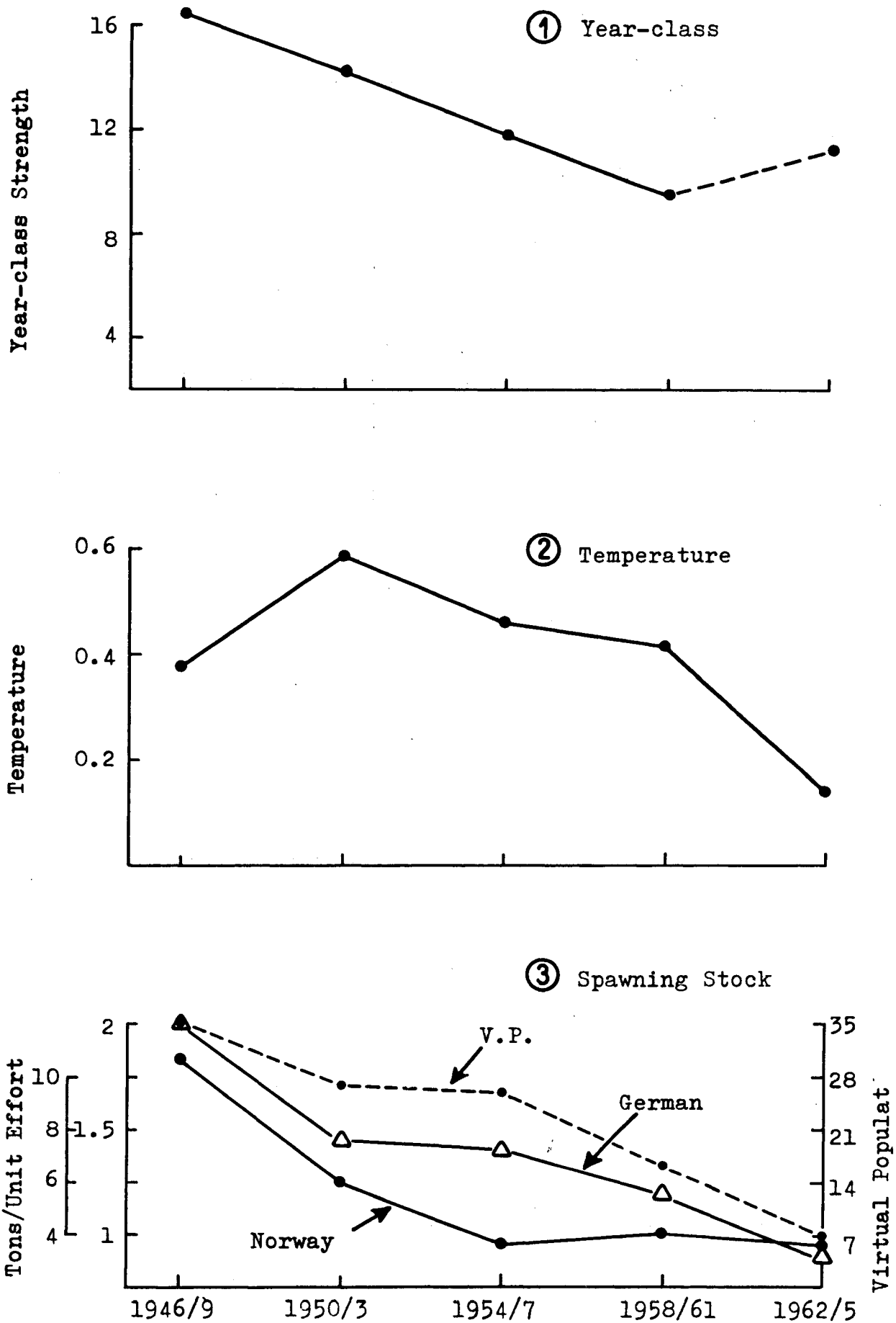
Figure 5. Fluctuations in Year-class, Temperature and Spawning Stock.
