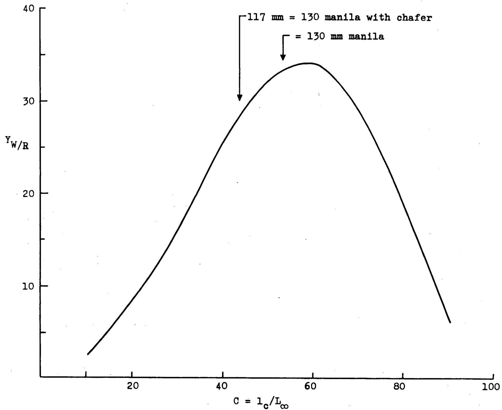
Figure 7. H. DOCK. Changes in yield per recruit with mesh-size.
